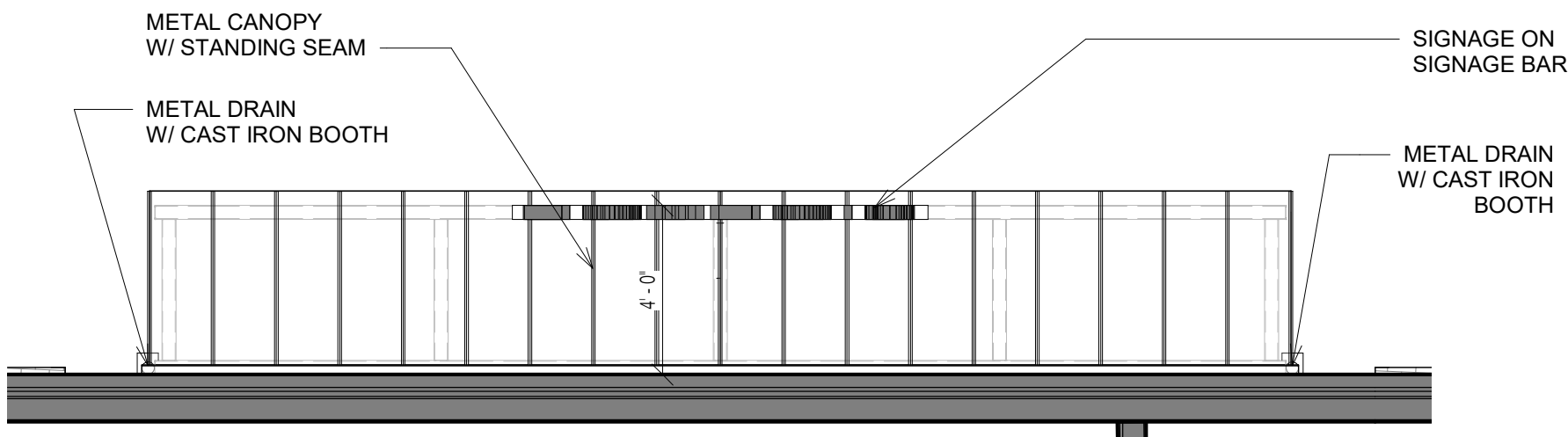
5 SIGNAGE PLAN VIEW 1/4" = 1'-0"
