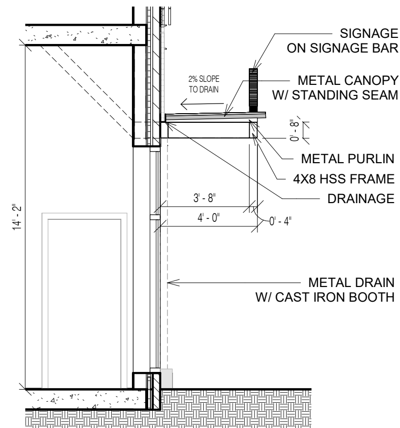
2 SIGNAGE SECTION DETAIL 1/4" = 1'-0"
